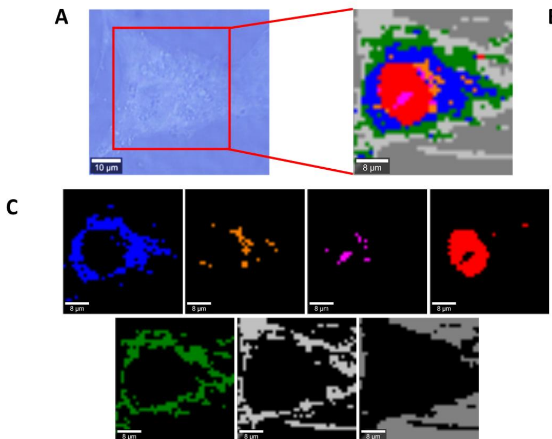
Figure 1. Microscopy image (A), Raman image of glioblastoma (U-87 MG) cell ( 30 \times 20 \mu\text{m} , resolution 1.0 \mu\text{m} ) incubated with Pfizer/BioNT vaccine (dose 60 \mu\text{L}/\text{mL} ) for 96 hours (B) and Raman images of specific organelles: lipids and lipid droplets (blue and orange), mitochondria (magenta), nucleus (red), cytoplasm (green), membrane (light grey), cell environment (dark grey) at 532 \text{ nm} .
