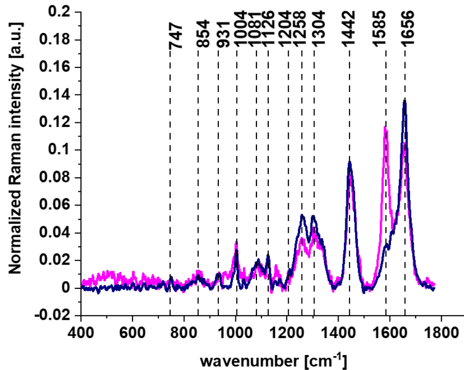
419 Figure 6. Average Raman spectra for mitochondria for glioblastoma U87-MG cells without (violet) and 420 upon incubation for 24h with retinoic acid ( c=50\ \mu\text{M} , pink), (alle spectra represent the arithmetic mean of 421 3 spectra characteristic for mitochondria of analyzed cells, calculated based on the minimum 1600 single 422 Raman spectra, excitation wavelength 532 nm, laser power 10 mW, integration time 1.0 sec).
